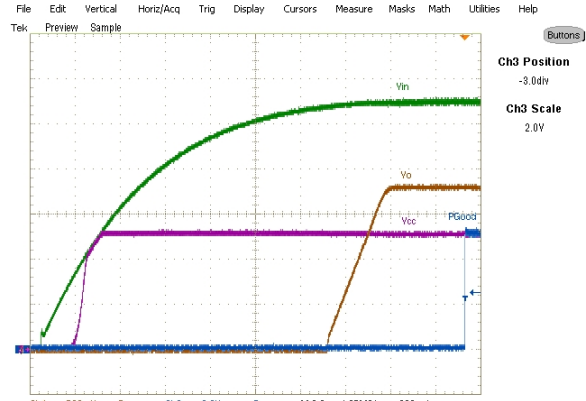
Fig. 10: Start up at 14A Load (Note 1) Ch 1 :V out Ch 2 :PGood Ch 3 :V cc Ch 4 : V in
