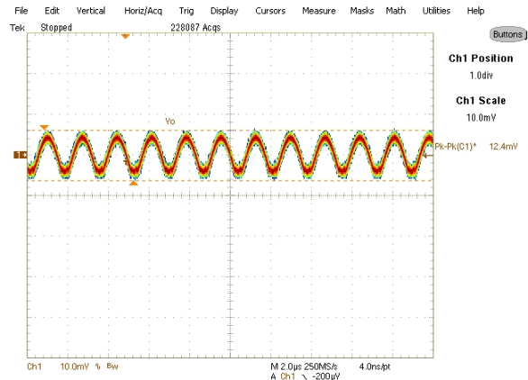
Fig. 12: Output Voltage Ripple, 14A load (Note2) Ch 1 : V out
